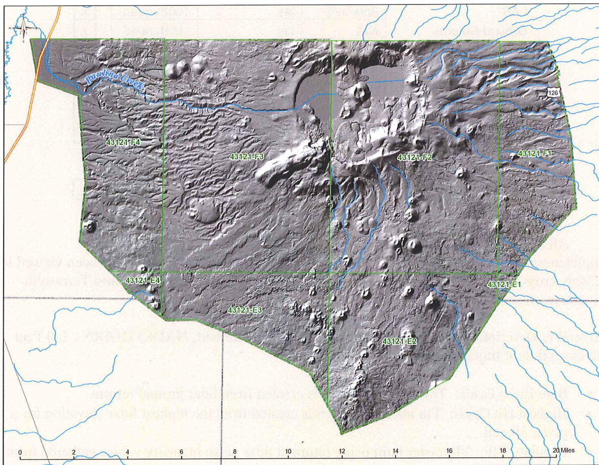
Figure 1. Delivery 3 location area. Data is referenced to USGS 7.5 minute quadrangles within the extents of the Newberry CVO Survey collection area.
