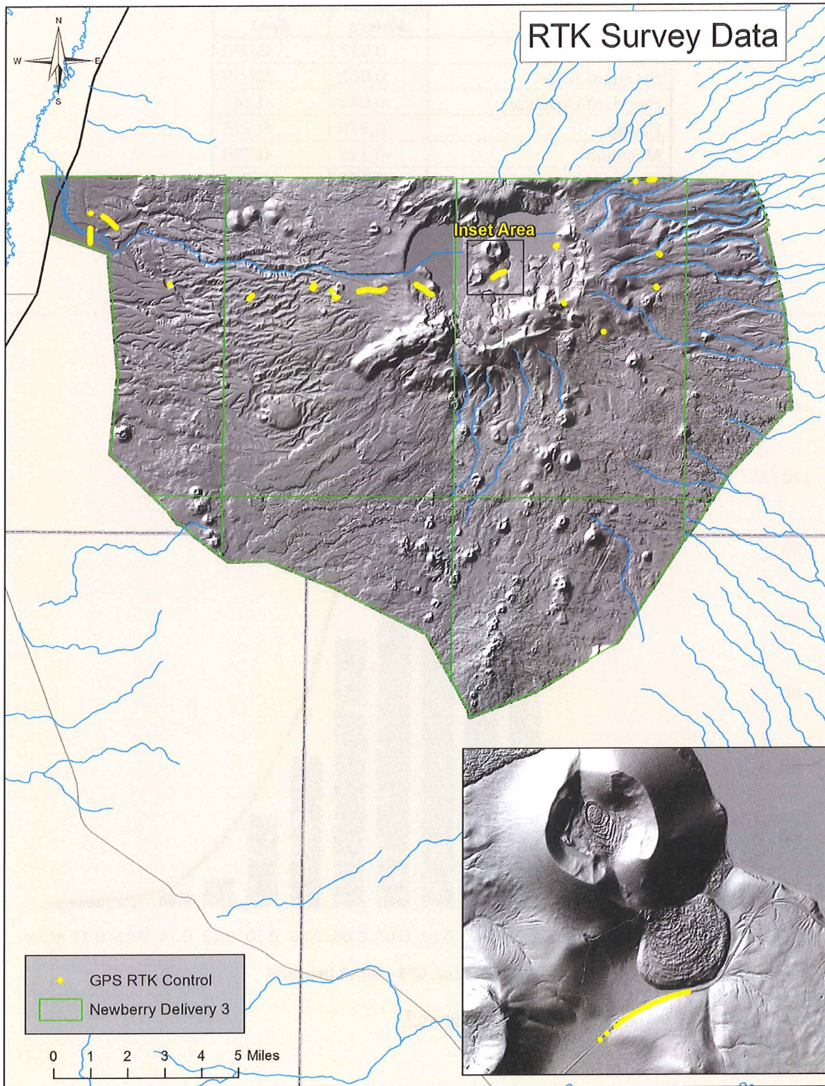
Figure 6. Locations of RTK control surveyed by DOGAMI. Data was used to test absolute accuracy for the Newberry CVO lidar survey within the Delivery 3 extent.
